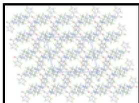
Fig. 3. Unit-cell contents for (I) shown in projection down the b axis. The N—H...O hydrogen bonds and C—H... \pi interactions are shown as blue and purple dashed lines, respectively.
