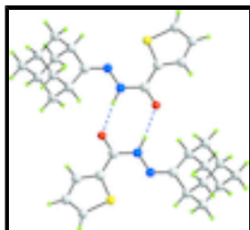
Fig. 2. Centrosymmetric dimer in (I) sustained by N—H...O hydrogen bonds shown as blue dashed lines.
