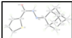
Fig. 1. The molecular structure of (I) showing the atom-labelling scheme and displacement ellipsoids at the 50% probability level. Only the major component of the disordered thiophene ring is shown for reasons of clarity.
